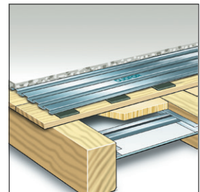
Woningscheidend / brandwerend
